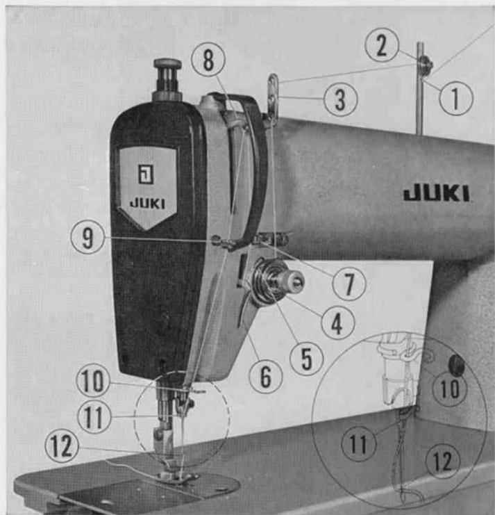
Fig. 14 Threading the machine
