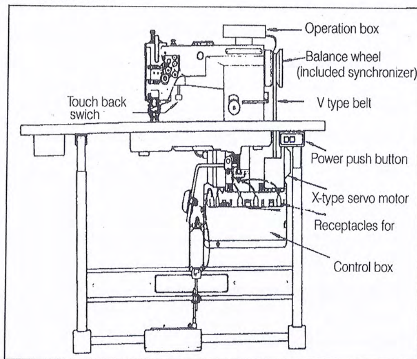
Overall view of assembled sewing machine
