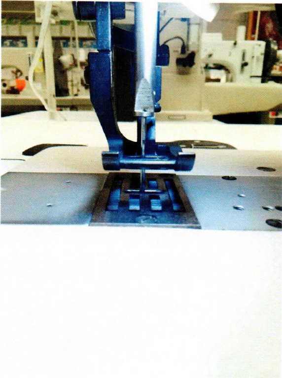
Lateral Setting of Straight Stitch.
