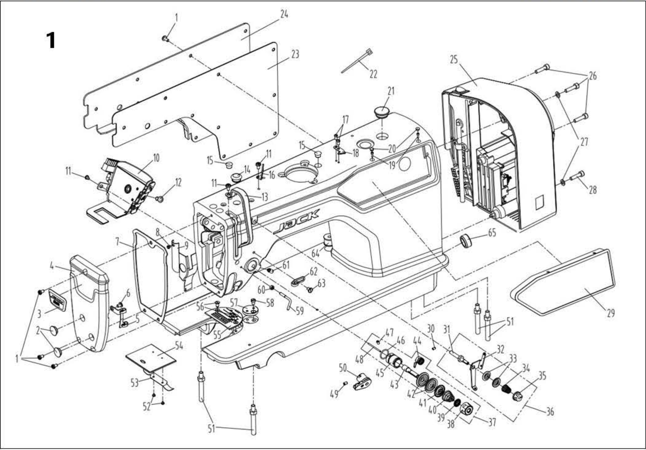
1. 机壳、外装部件/Machine Frame & Miscellaneous Cover Components
