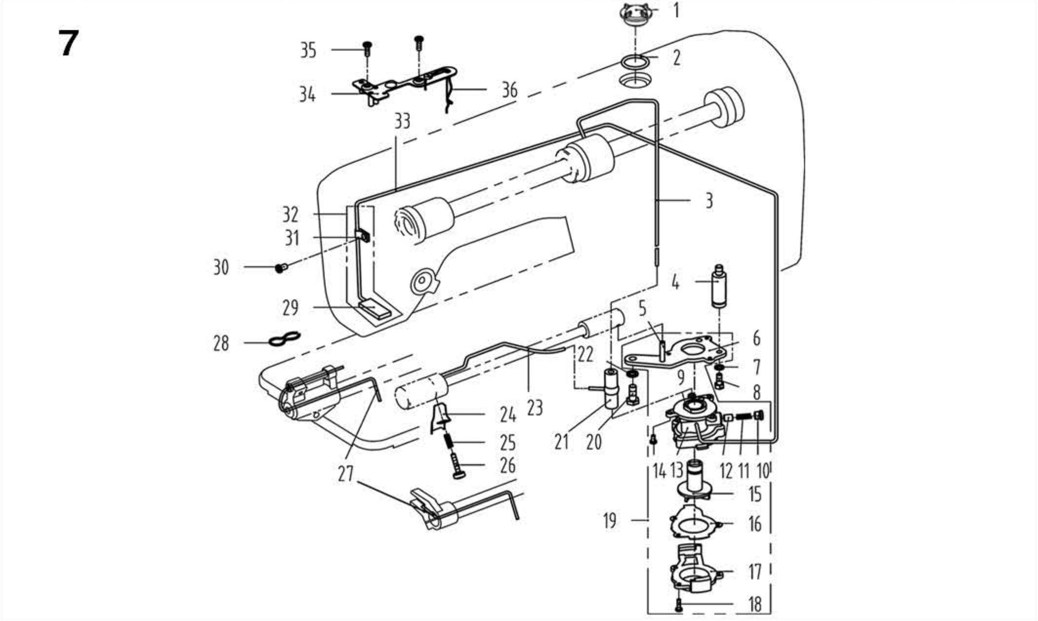
7. 润滑部件/Oil Lubrication Components(1)
