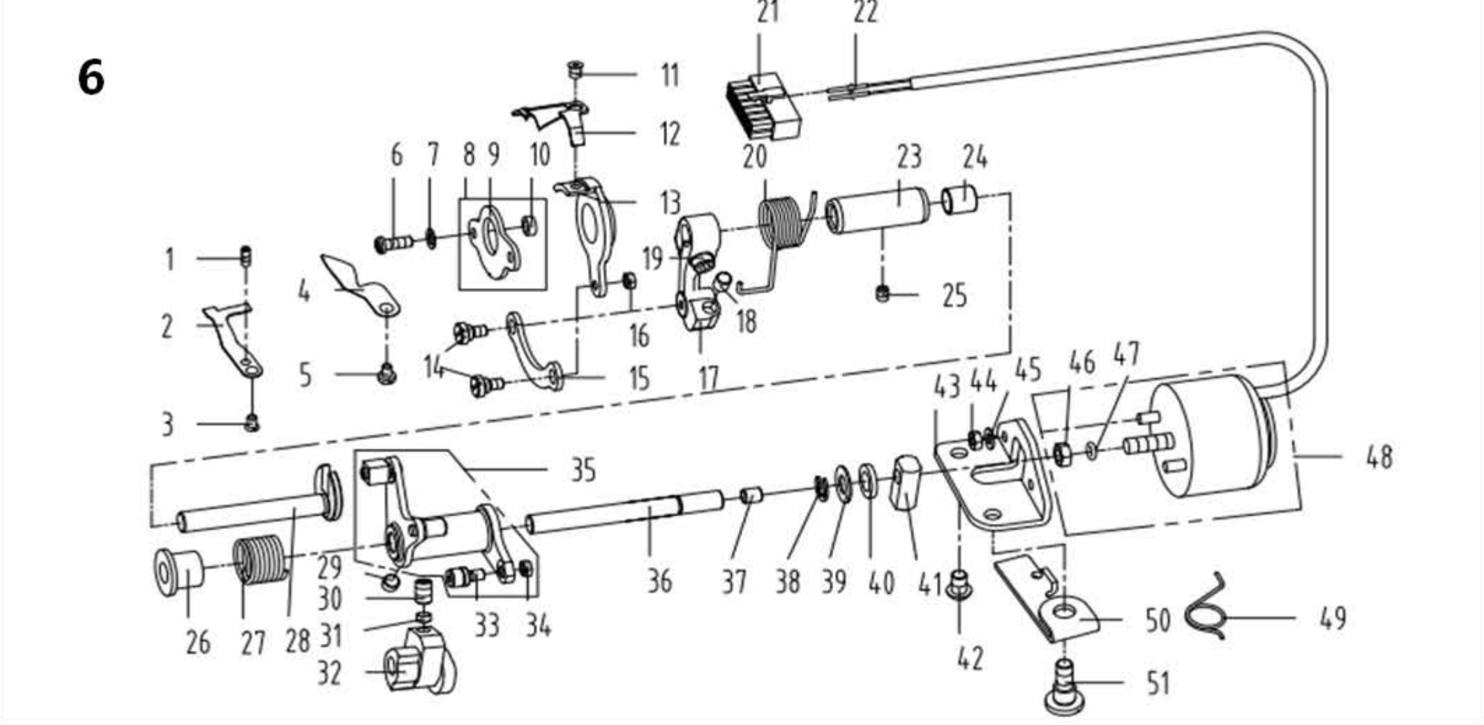
6. 切线装置部件/Thread Trimmer Components
