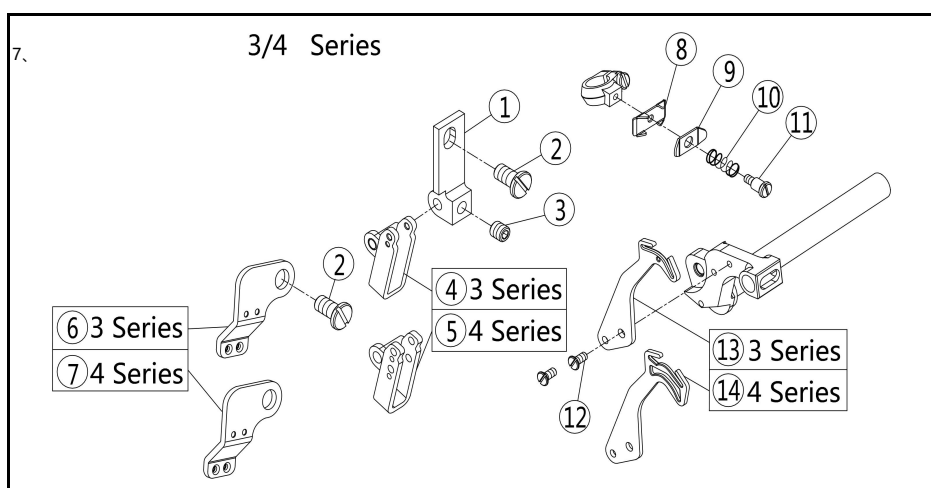
七、过线机构(2)/Thread Guide and Thread Takeup(2)
