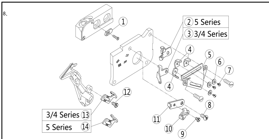
八、过线机构(3)/Thread Guide and Thread Takeup(3)
