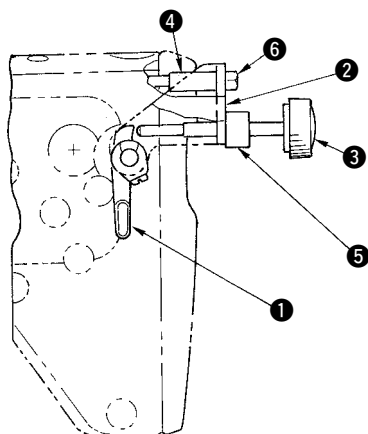
Presser foot micro-lifter components
