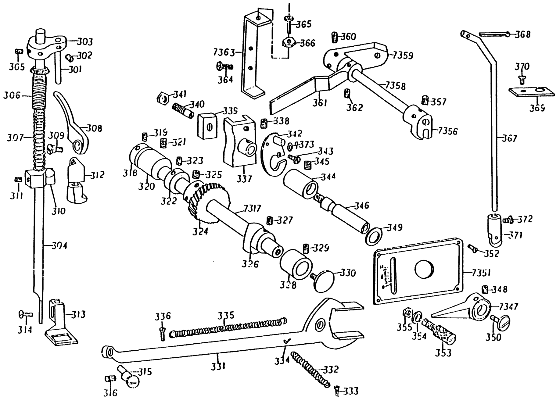
Fig. 7-27: Zigzag Width Regulating Mechanism Components & Presser Bar Assembly
