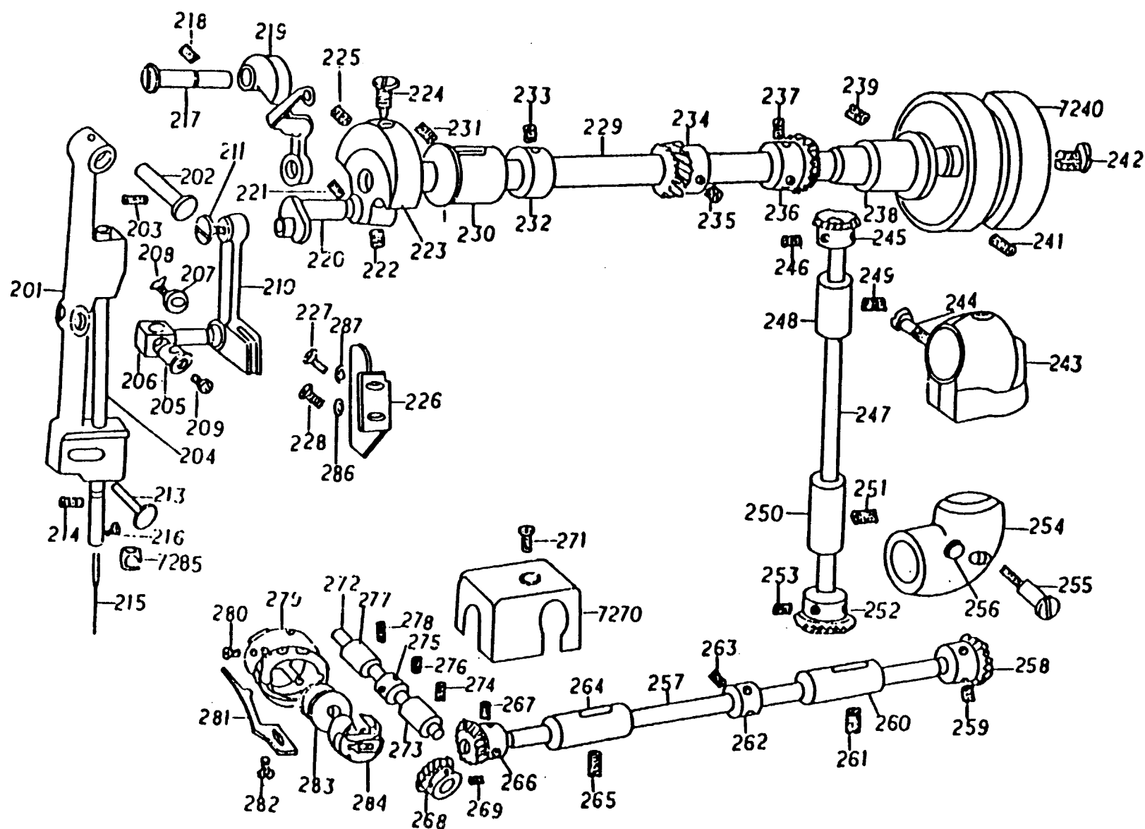
Fig. 7-26: Needle Bar and Hook Drive Shaft Components
