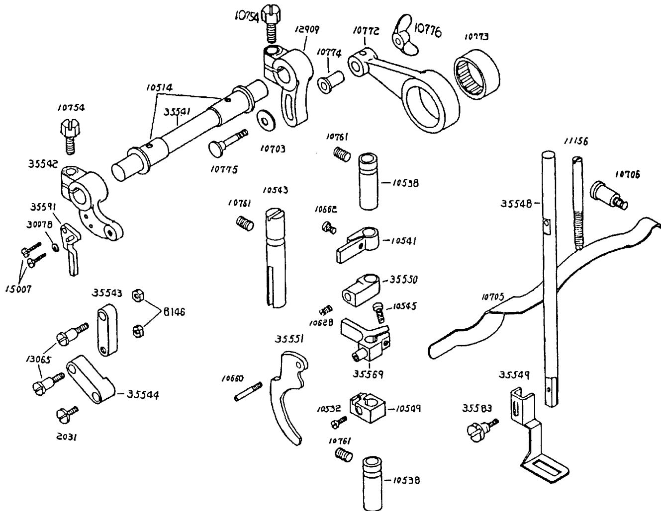
Presser Bar & Components - fig. 20
