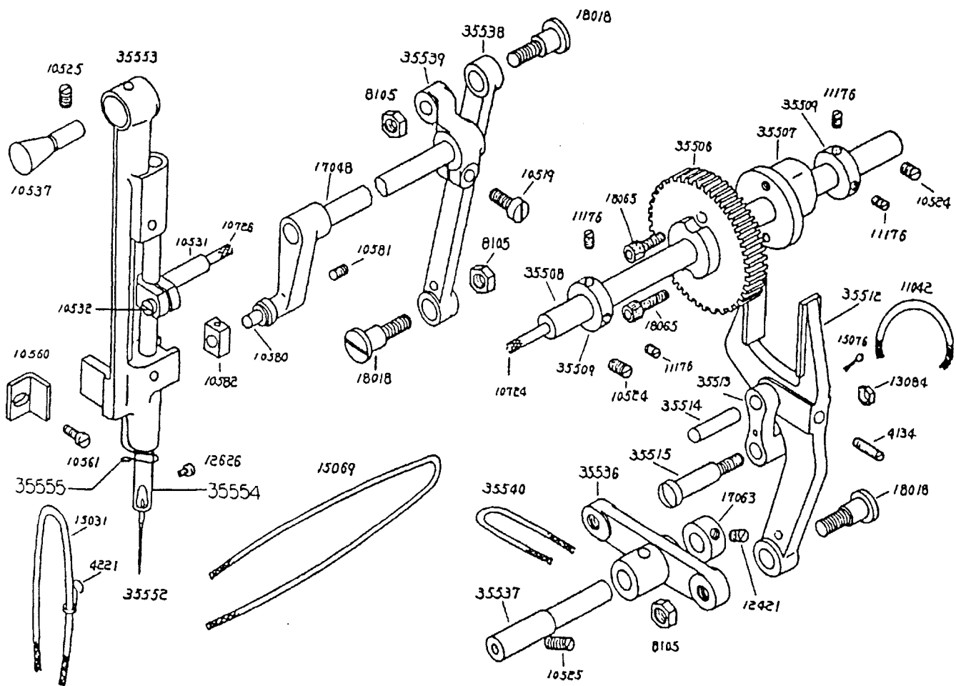
XL Sewing Head Needle Bar - fig. 18
