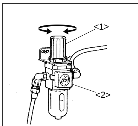
<1>: Adjusting knob <2>: Air regulator
