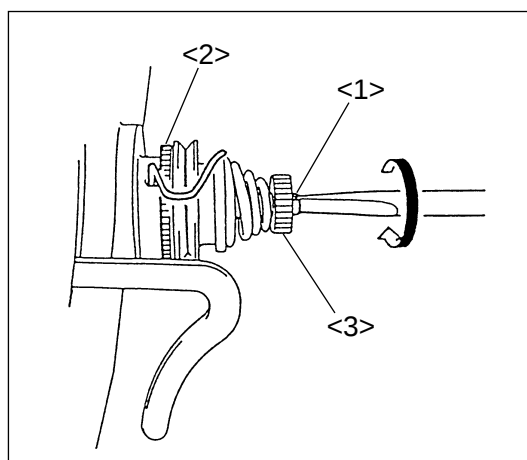
<1>: Adjusting shaft <2>: Adjusting bushing <3>: Adjusting nut
