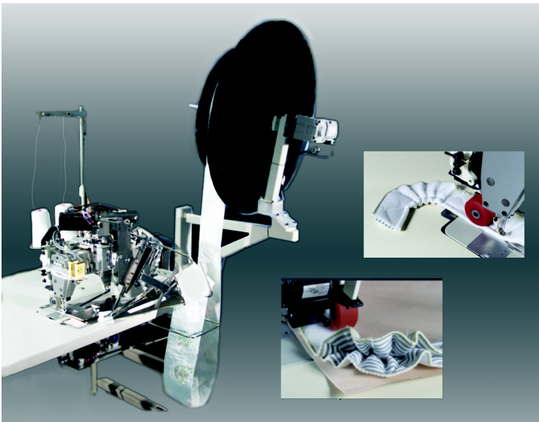
GPT-1000 Ruffler Machine
