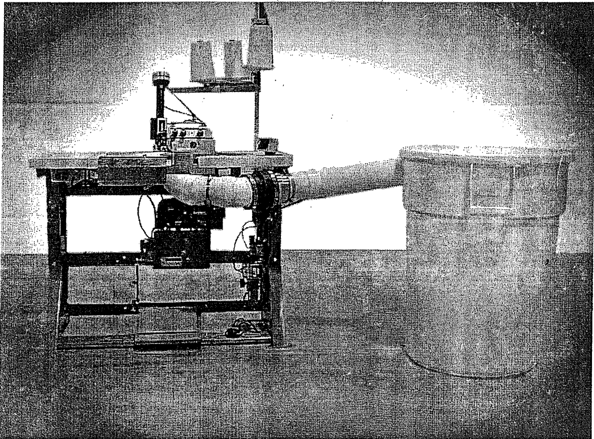
PFM-2002 Flange Machine
