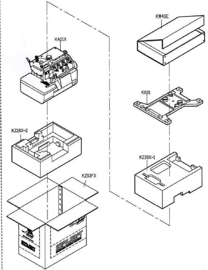
PARTS LIST FOR KZ GROUP
