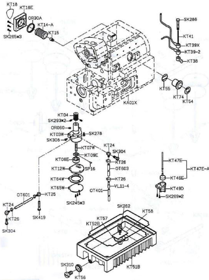
PARTS LIST FOR KT GROUP
