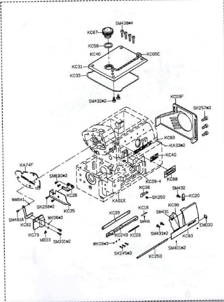
PARTS LIST FOR KC GROUP
