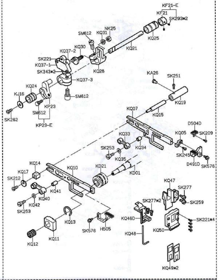
PARTS LIST FOR KQ GROUP
