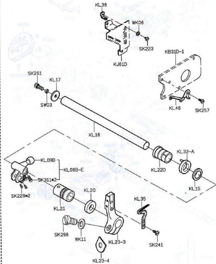
PARTS LIST FOR KL GROUP
