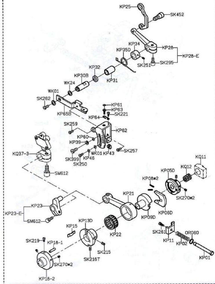
PARTS LIST FOR KP GROUP
