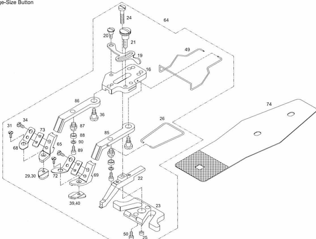
◎Parts for Large-Size Button
