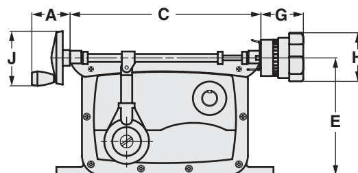
Type MD-RH
